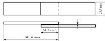
Gambar 1. Sambungan tumpang/lap joint ASTM 5868-95
