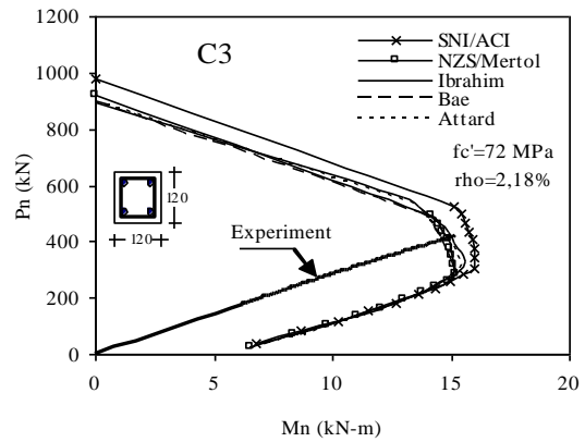
(b) Column C3; \rho=2.18\% , e/h=0.42
