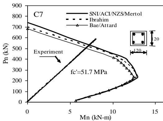
(a) Column C7; \rho=2.18\% , e/h=0.21
