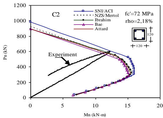
(a) Column C2; \rho=2.18\% , e/h=0.21
