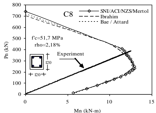
(b) Column C8; \rho=2.18\% , e/h=0.42
