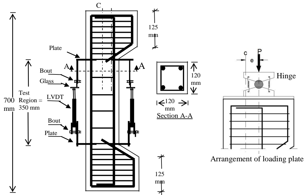
Figure 2. Detail of column specimens
