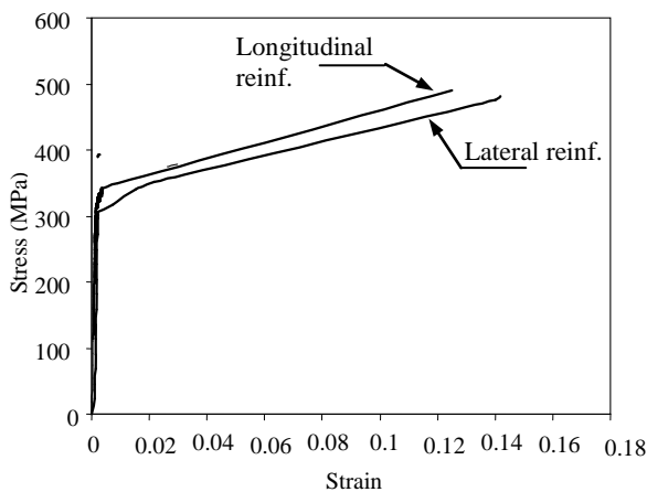
Figure 1. Stress-strain curves of lateral and longitudinal reinforcement
