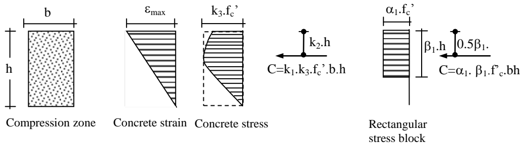
Figure 4. Stress block parameters
