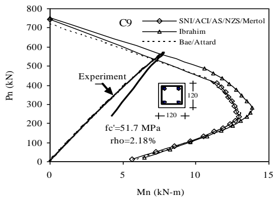
(c) Column C9; \rho=2.18\% , e/h=0.21
