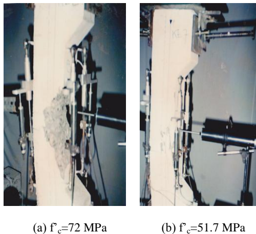
Figure 3. Failure of columns
