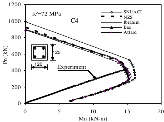
(c) Column C4; \rho=2.18\% , e/h=0.21
