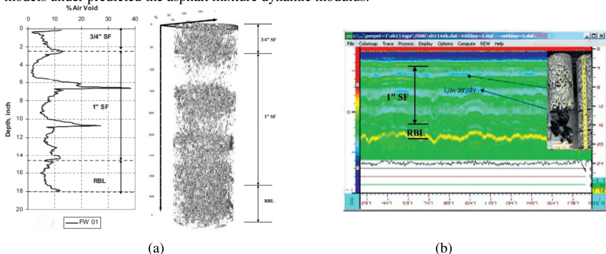
Picture 5. Three-Dimensional Images of Air Void and the percentage Air Voids Distribution plot (a), and GPR Data (b) (Kassem et al. 2008).
