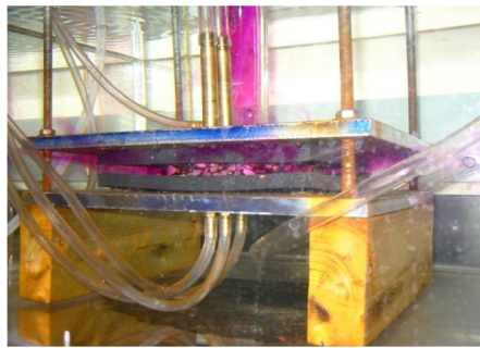
Picture 6. Setup of the Testing Apparatus
