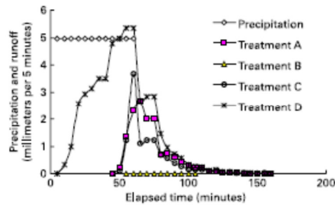
Picture 9. Comparison of precipitation rate, surface runoff of three porous pavement cells and the impervious surface cell.
