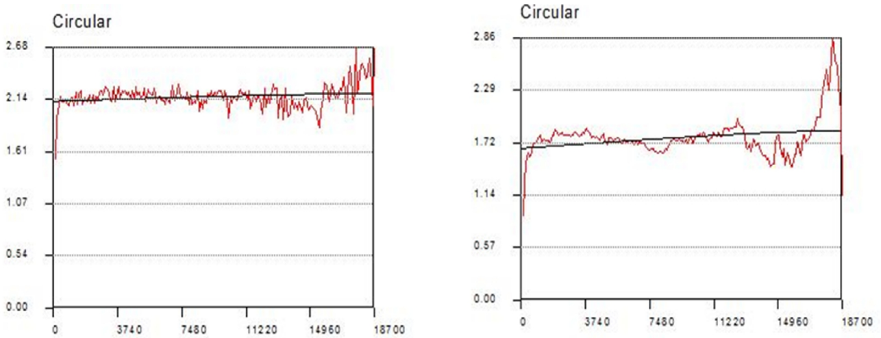
Figure 2 Semivariogram in Run up scenario
