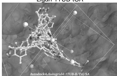
Ligan-1TUB-SA
