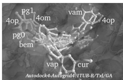
Ligan-1TUB-tGA
