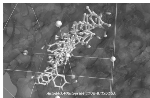
Ligan-1TUB-LGA
